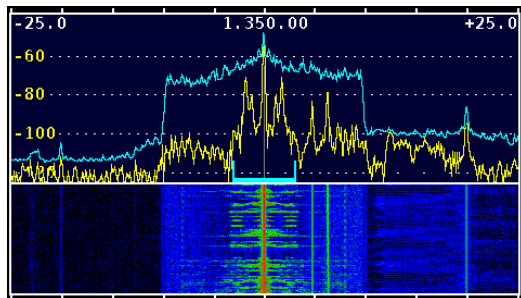
Figure 17. Typical AM Spectra using Peak Hold.
