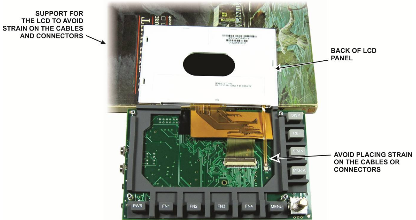
Figure 47. Removing LCD Panel from Rubber Key Matrix.
