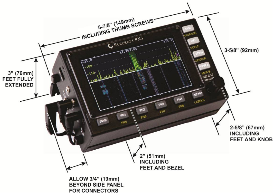
Figure 49. PX3 Dimensions.
