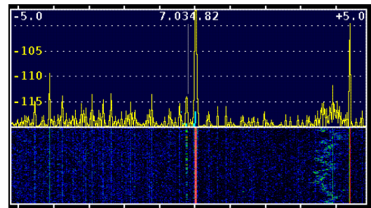
Figure 15. Typical Spectra Display.
